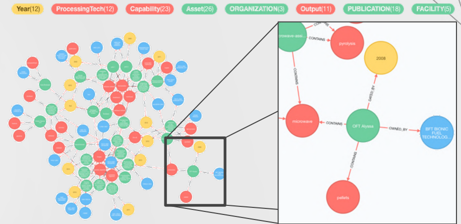
Knowledge Graph
